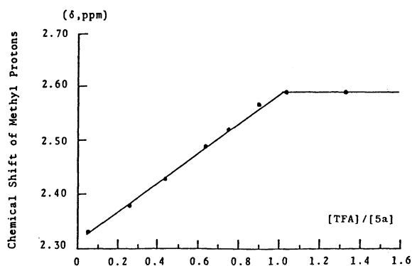
Fig. 2. Relation of chemical shift of methyl protons in 5a and the amount of added TFA ( \text{CD}_2\text{Cl}_2 ). [\mathbf{5a}] = 0.3\text{--}0.4\text{ M} .
